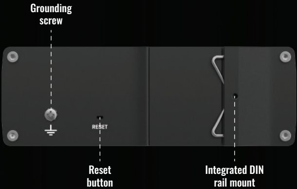
BACK VIEW
